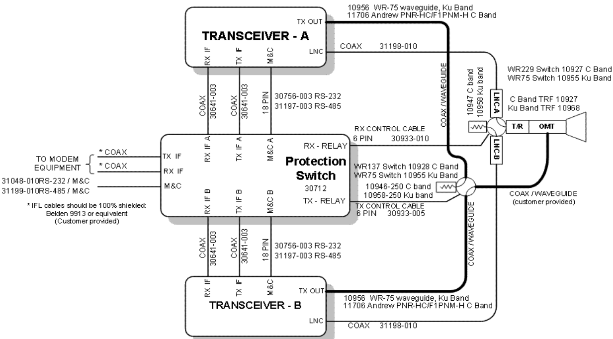
ANACOM 1 + 1 Redundancy Protection Switch Cabling Diagram (C Band, Single Enclosure) (Ku Band, Single Enclosure)
