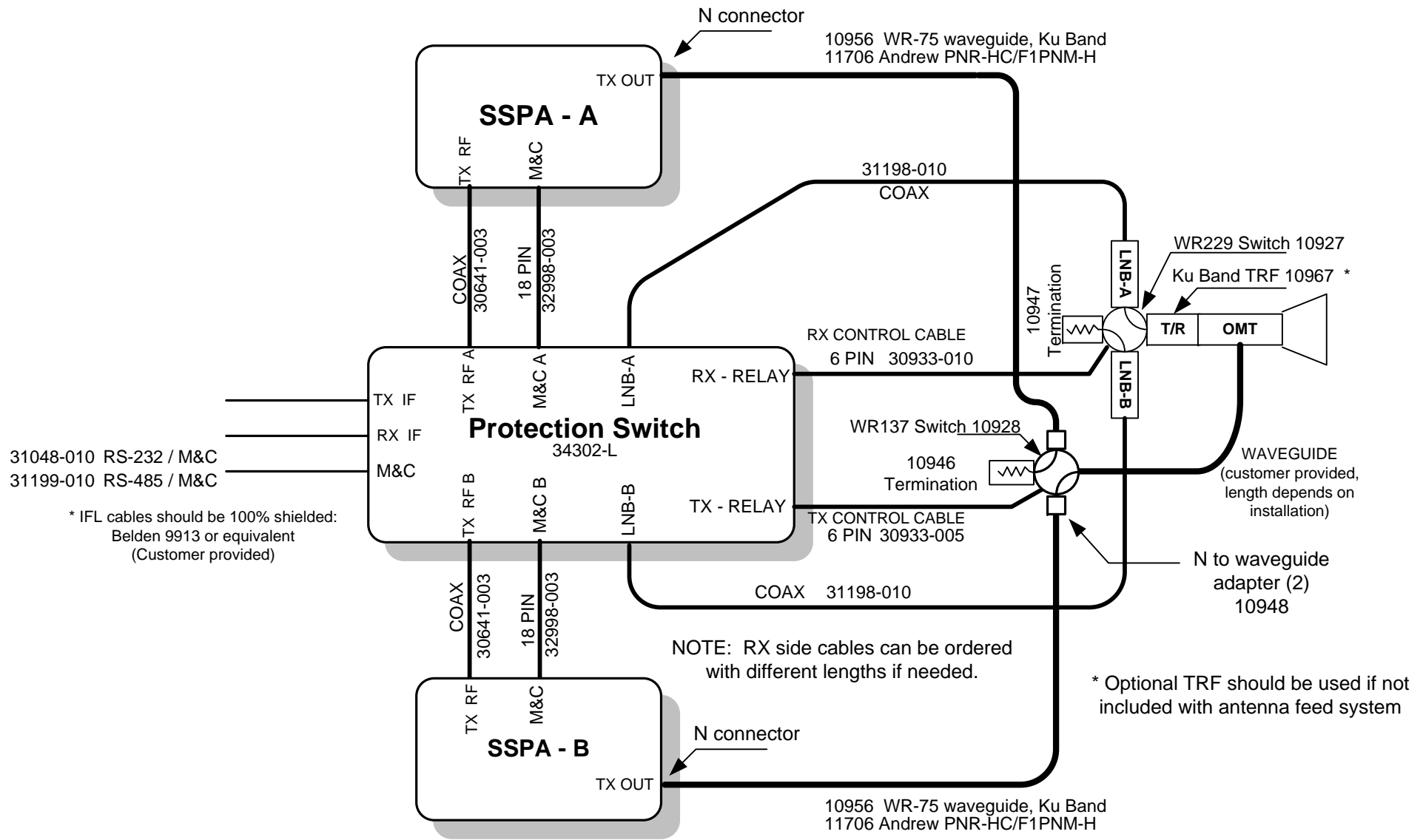
ANACOM 1 + 1 Redundancy Protection Switch Cabling Diagram (Ku Band, SSPA + LNB)
